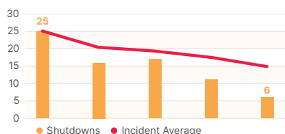
Incident Tracker
